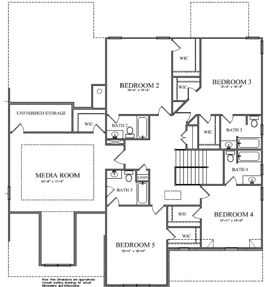
SECOND FLOOR PLAN BAINBRIDGE B
