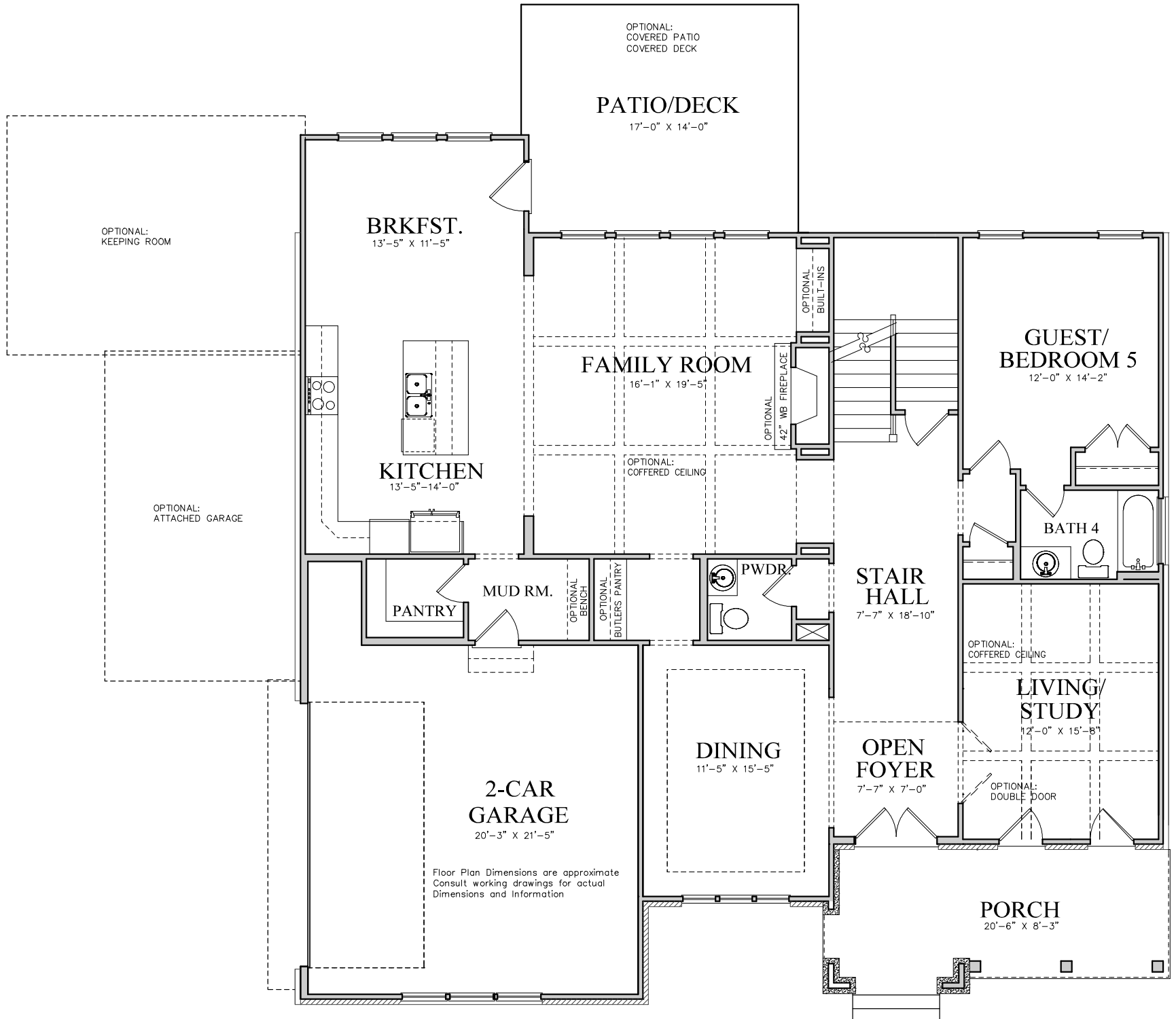
FIRST FLOOR PLAN DILLARD C
